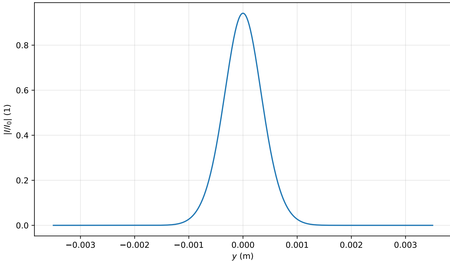
Intensity profile I(x=0, y, z=0.955)/I_0 , P_{in}=0.3P_{cr} , artificial time
